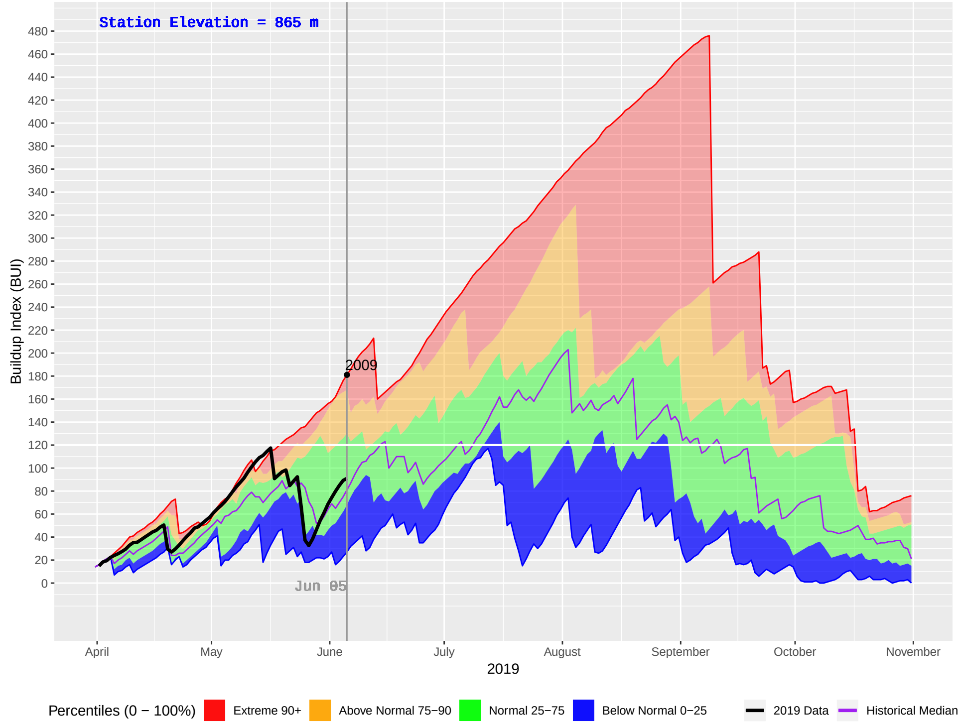
FIVE MILE (1029) : Historical (2008–2018), Current (2019) Daily Buildup Index (BUI)
