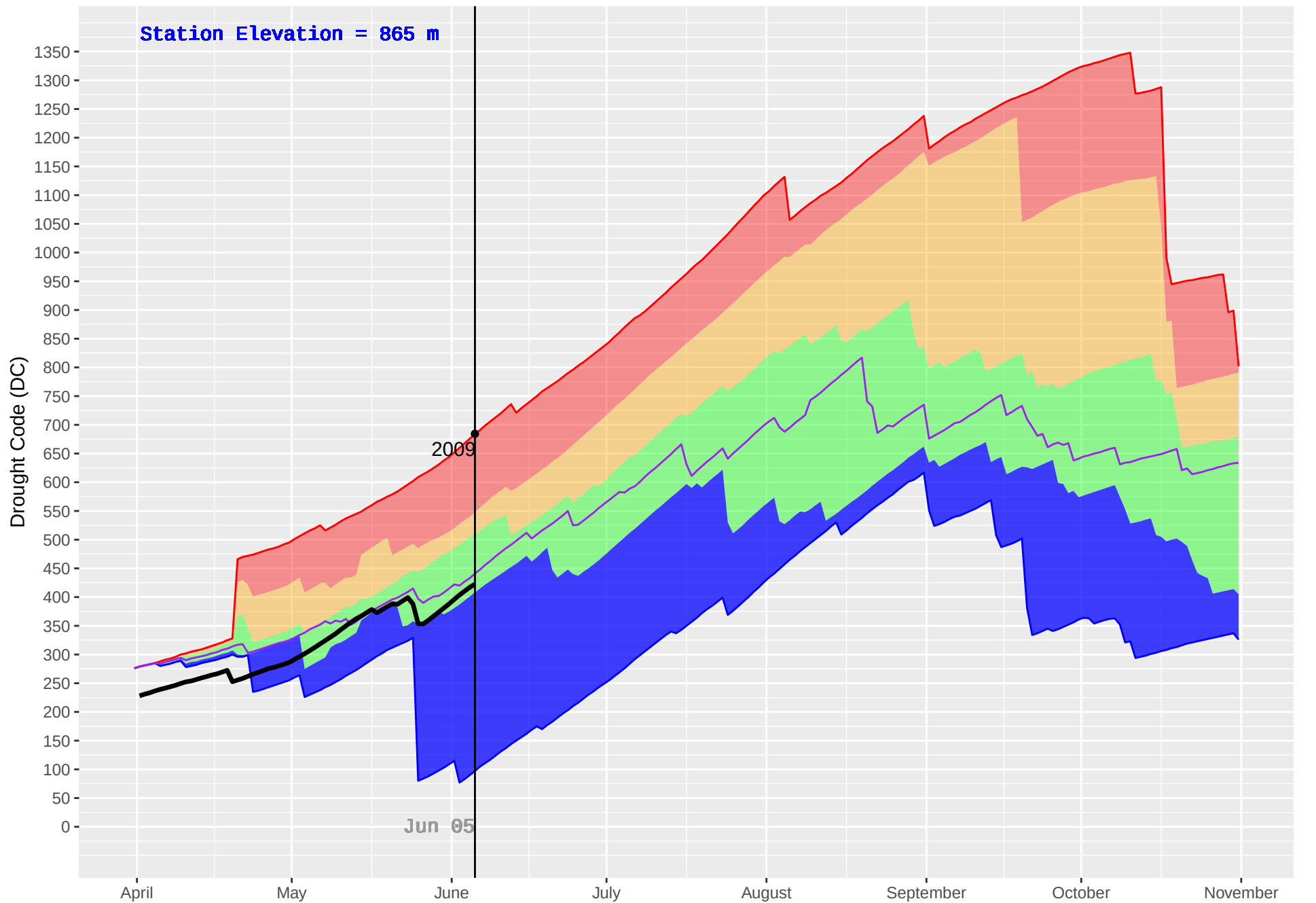
FIVE MILE (1029) : Historical (2008–2018) and Current (2019) Daily Drought Code (DC)
