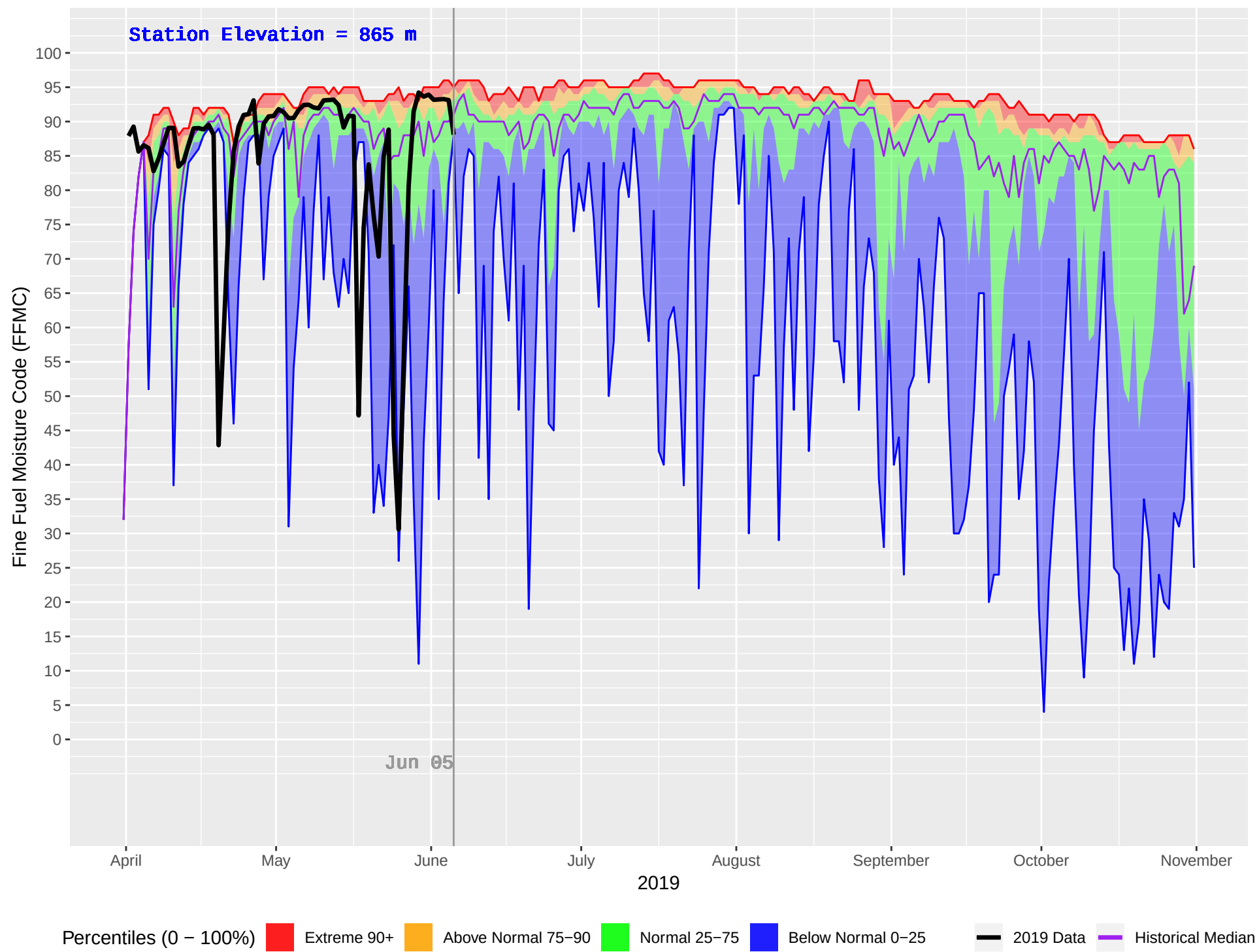
FIVE MILE (1029) : Historical (2008–2018) and Current (2019) Daily Fine Fuel Moisture Code (FFMC)
