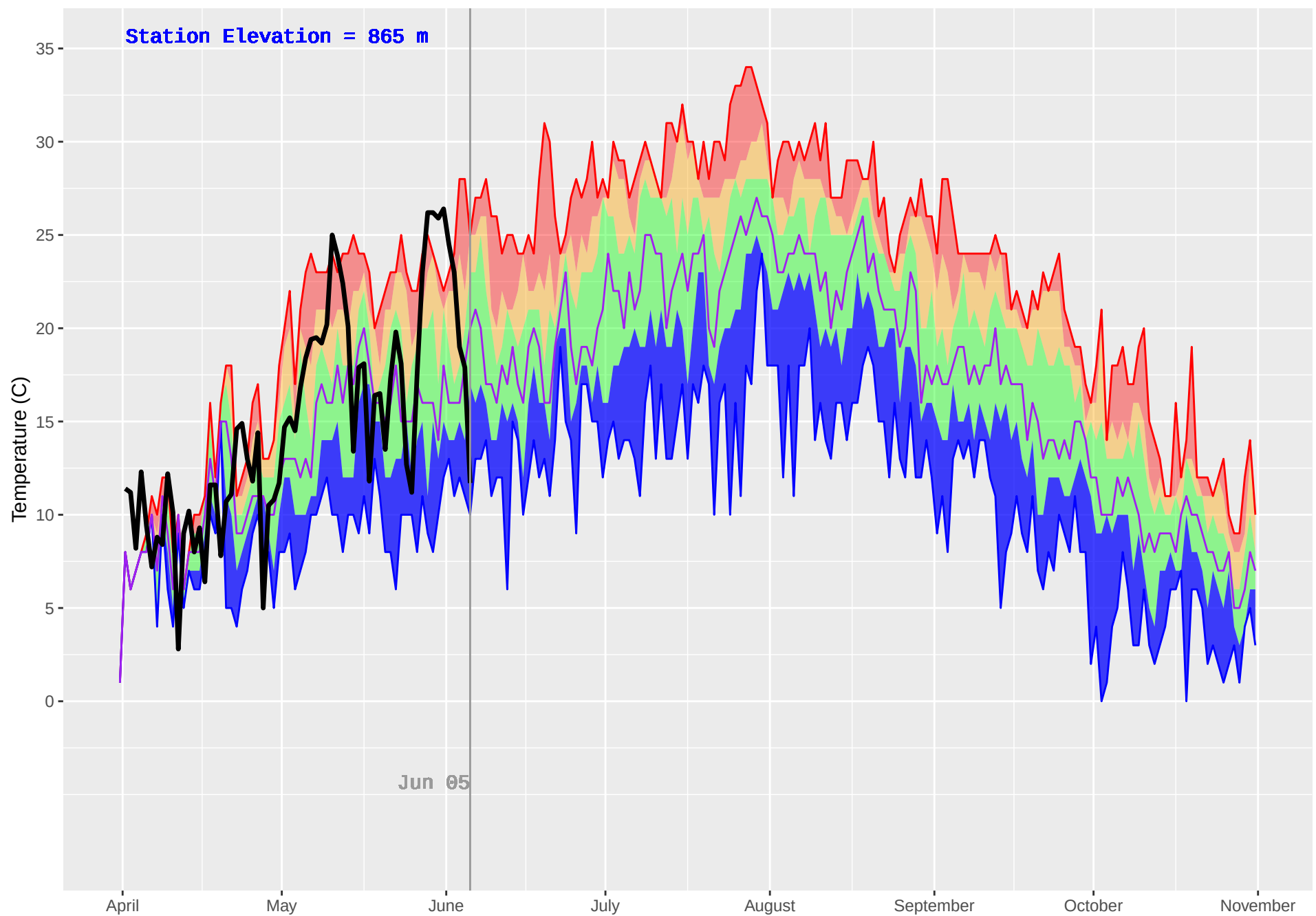
FIVE MILE (1029) : Historical (2008–2018) and Current (2019) Daily Temperature
