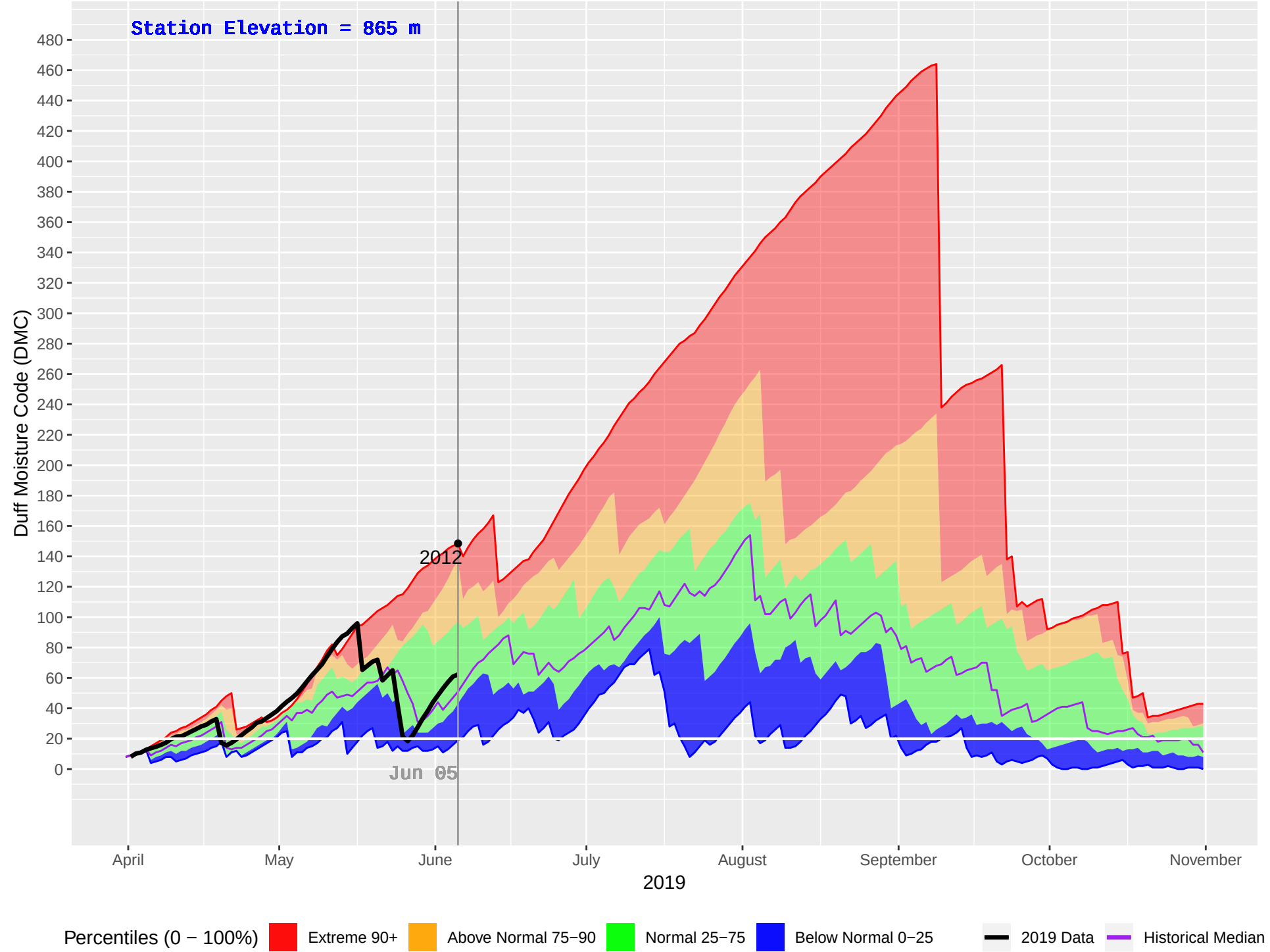
FIVE MILE (1029) : Historical (2008–2018), Current (2019) Daily Duff Moisture Code (DMC)
