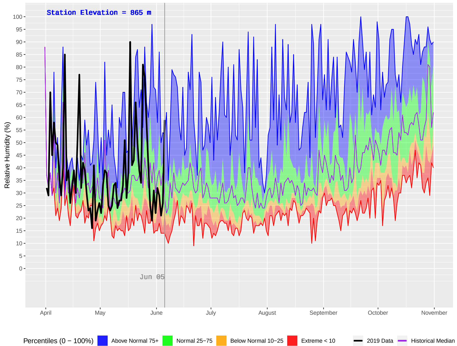
FIVE MILE (1029) : Historical (2008–2018) and Current (2019) Daily Relative Humidity
