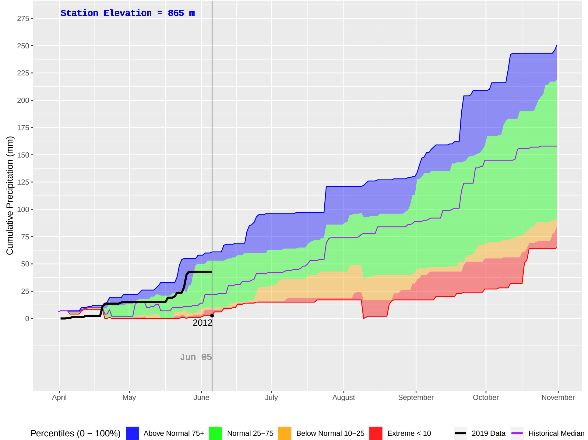
FIVE MILE (1029) : Historical (2008–2018), Current (2019) Daily Cumulative Precipitation
